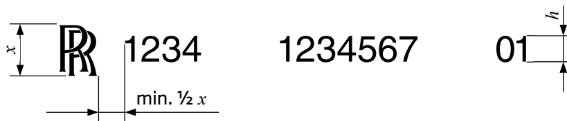
Figure 15: Marking with Rolls-Royce Motor Cars symbol and identification data version A
