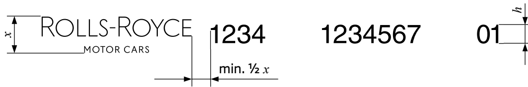
Figure 16: Marking with Rolls-Royce Motor Cars symbol and identification data version B
