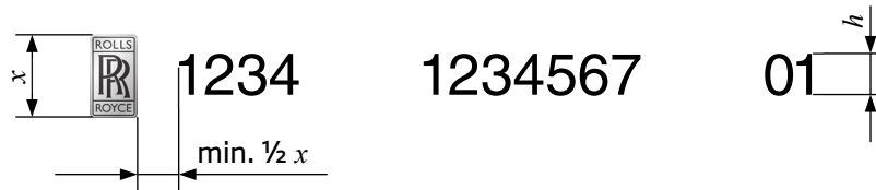
Figure 17: Marking with Rolls-Royce Motor Cars Badge of Honour and identification data version C
