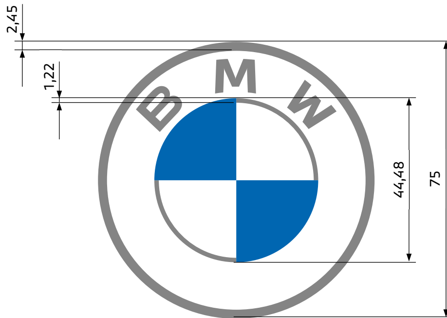
Figure 3: Dimensioning of the BMW symbol
