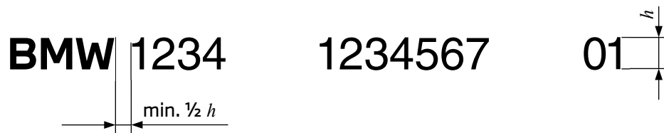
Figure 6: Marking with BMW symbol and identification data version B
